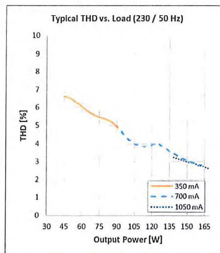
OT 165 4DIMLT2 G2 Typical THD vs Load
