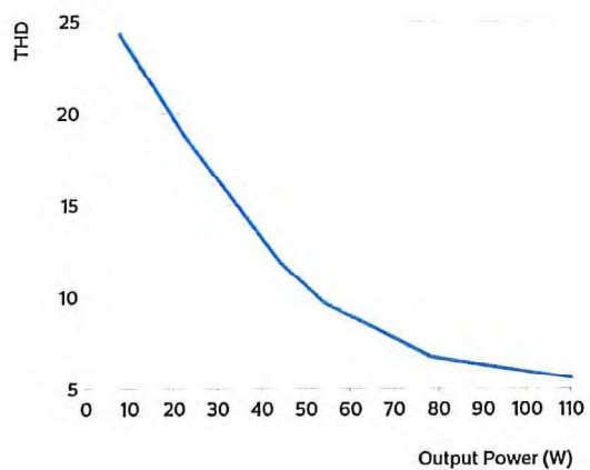
THD versus output power
